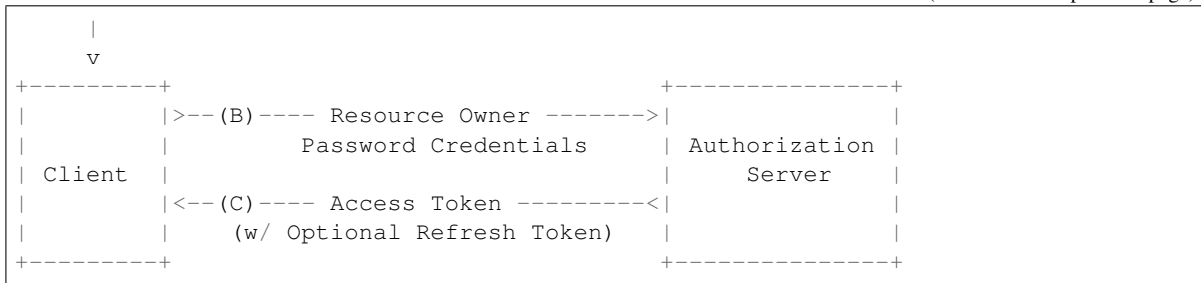
Figure 5: Resource Owner Password Credentials Flow
